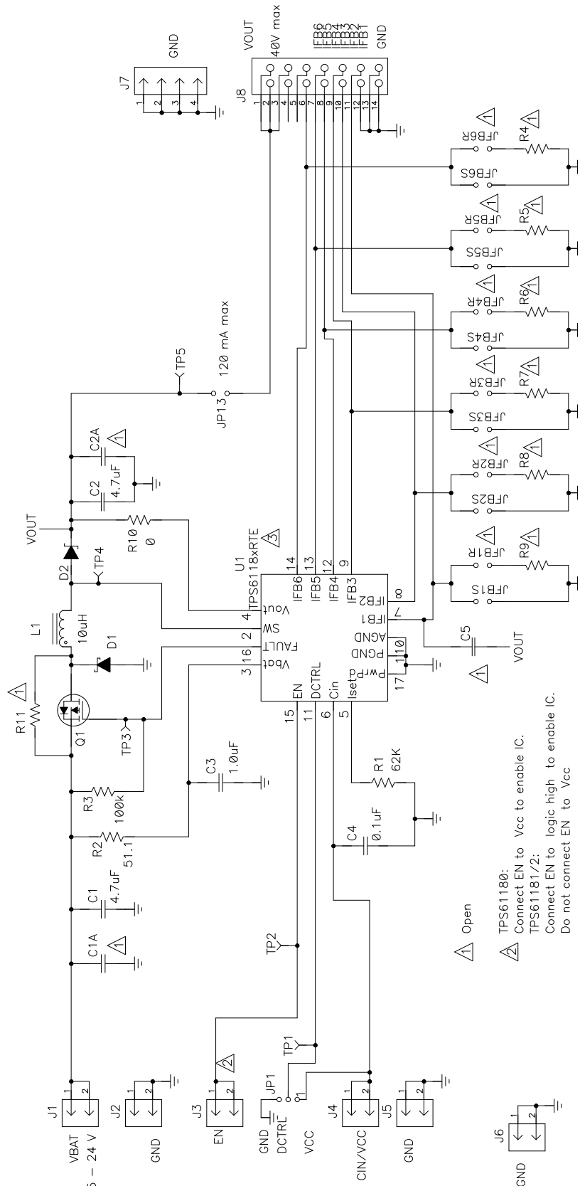
Figure 9. HPA259A Schematic
