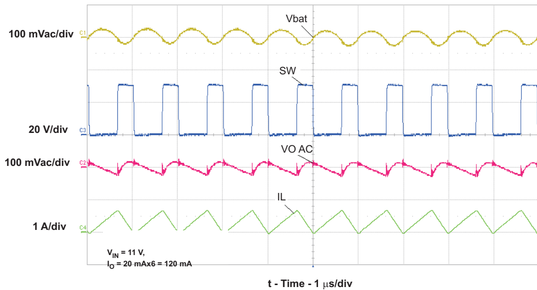
Figure 4. Switching Waveform
